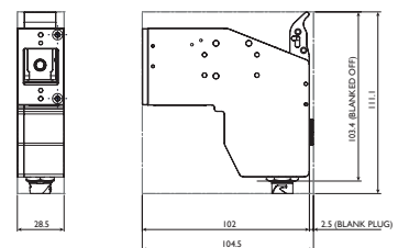
Compact printhead
