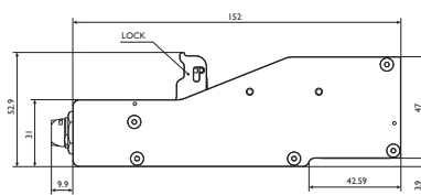
Standard printhead
